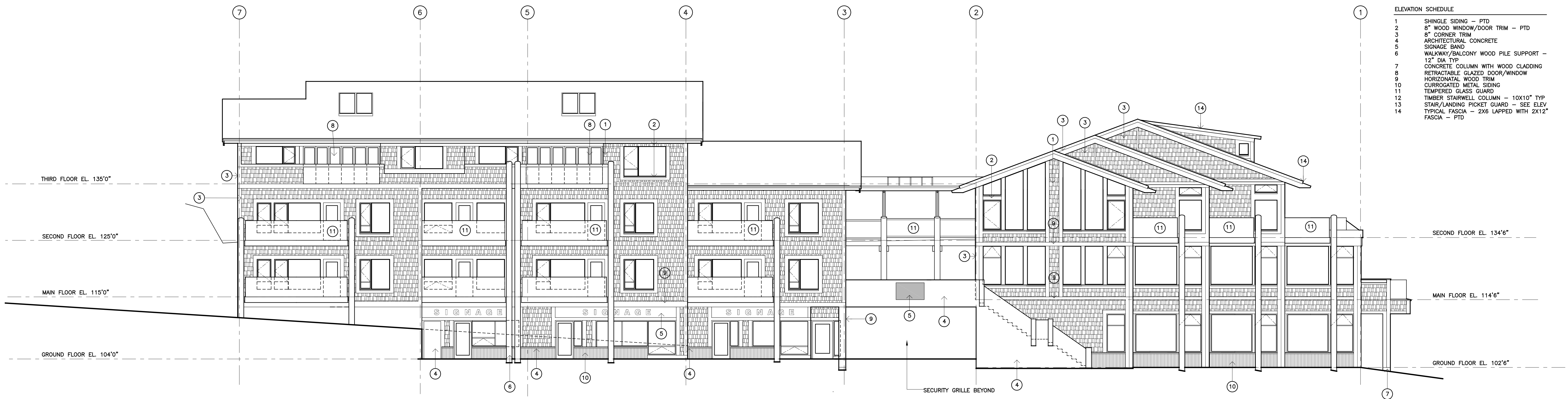
2 | NORTH ELEVATION - EAST AND WEST BUILDINGS
