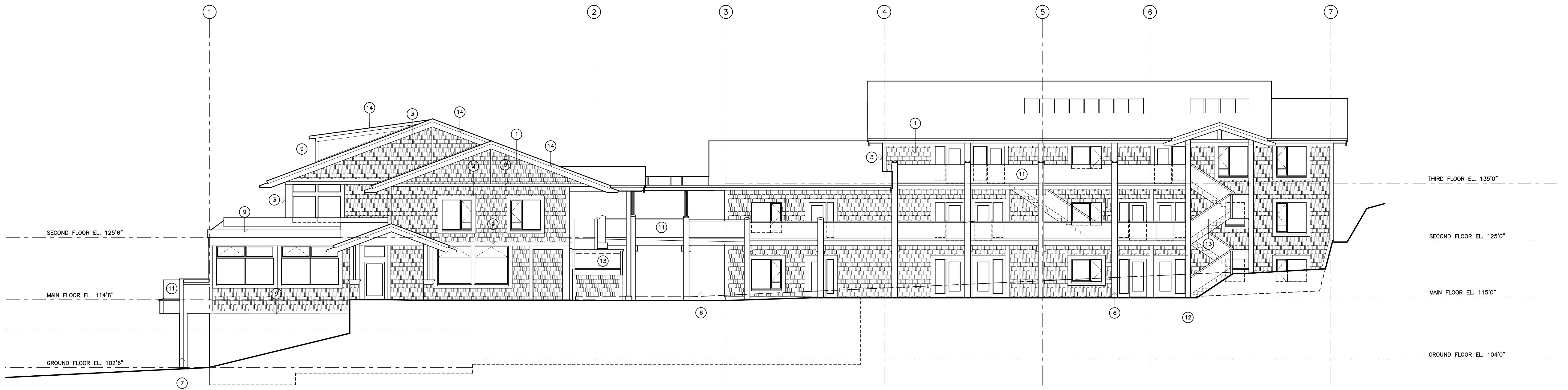
1 | SOUTH ELEVATION - EAST AND WEST BUILDINGS
