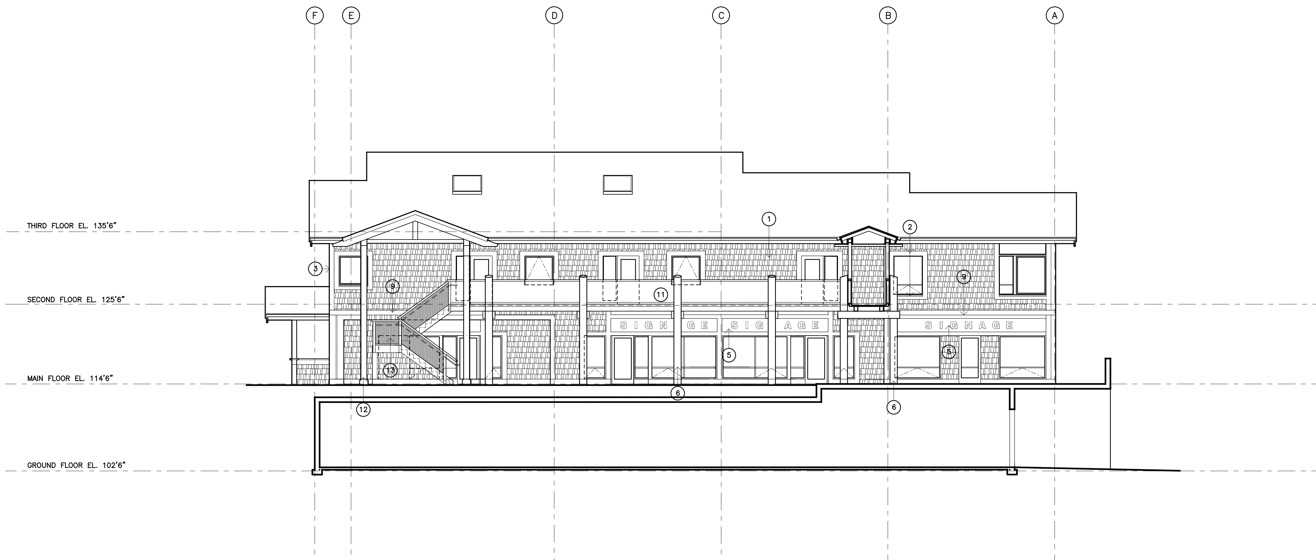
1 | EAST ELEVATION - WEST BUILDING A05 SCALE 1"=1/8"
