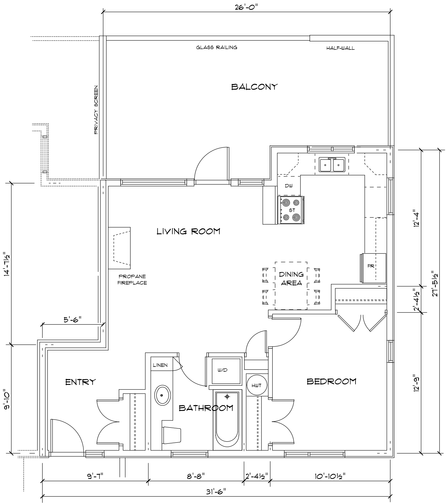
the Moorage STRATA LOT 14 FLOOR PLAN SCALE: 3/16" = 12" OCTOBER 21/07
