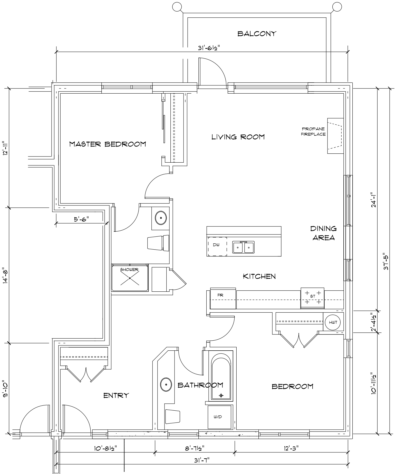
the Moorage STRATA LOT 8 FLOOR PLAN SCALE: 3/16" = 12" OCTOBER 12/07
